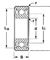
Shielded 2 Sides
